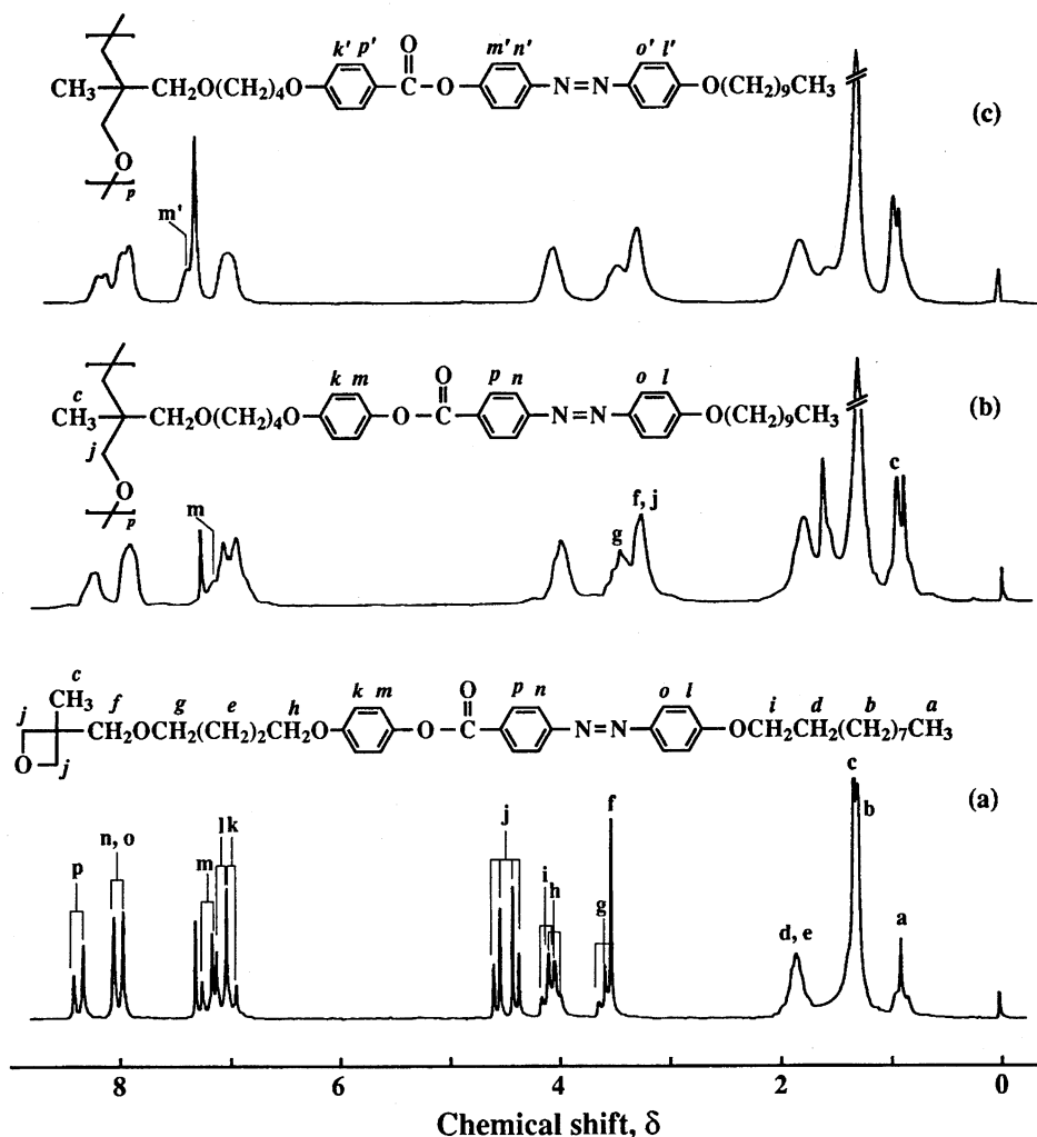
Fig. 2. 1 H NMR spectra of (a) 3d, (b) poly(3d), and (c) poly(2d).
