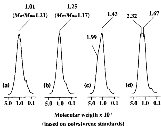
Fig. 1. GPC chromatograms of (a) poly(3a), (b) poly(3b), (c) poly(3c), and (d) poly(3d). Figures at peak tops indicate molecular weights ( \times 10^{-4} ) estimated from those of polystyrene standards.
